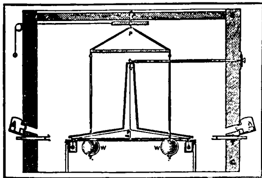
FIG. 2.—Cavendish's Apparatus.
