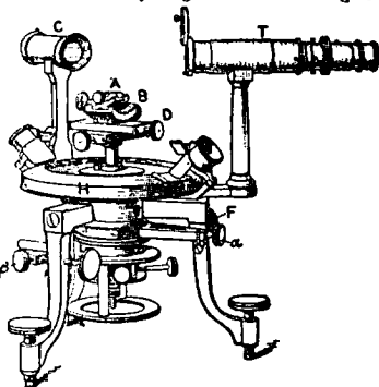
FIG. 3.—Horizontal-Circle Goniometer.
