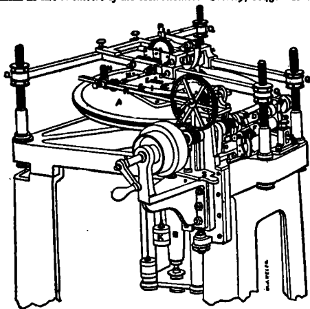
Dividing Engine.
